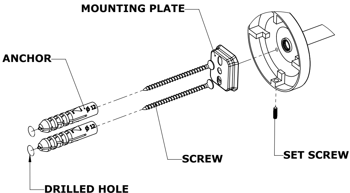
DETAIL M
